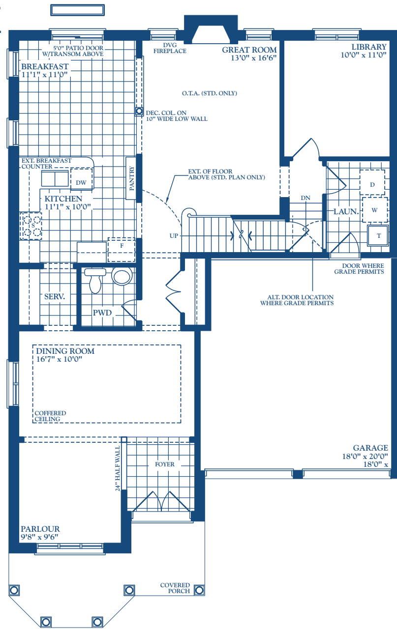
FIRST FLOOR ELEVATION A
