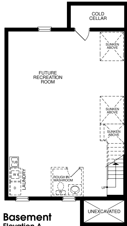
Basement Elevation A (BLK. 1 TH-4)
